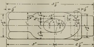
DETAILS OF COMBINATION HARD AND SOFT HAMMER.
